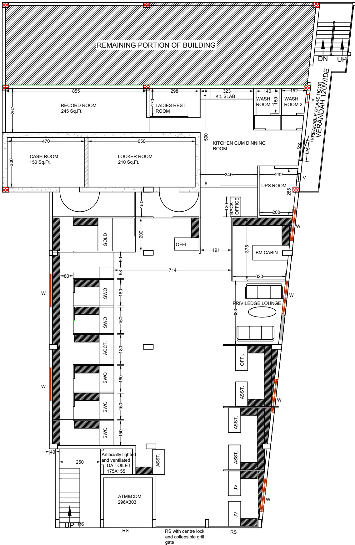
PROPOSED LAYOUT FOR SBI PERAMBRA ADB BUP AREA = 4146 Sq.Ft.
